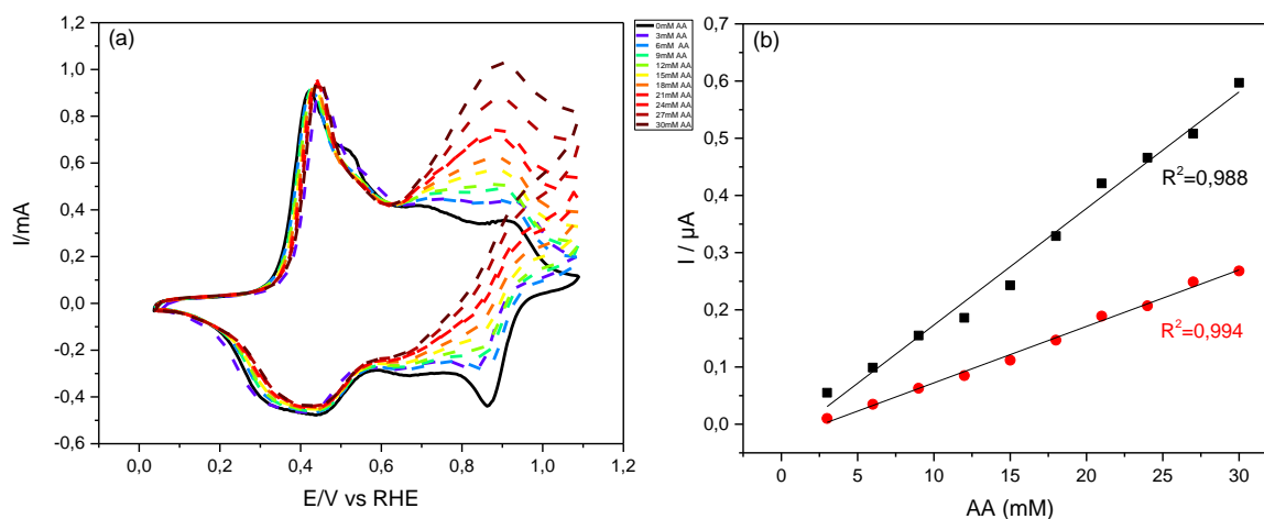
Figure.17 (a) cyclic voltammograms recorded during AA oxidation using a Pt electrode covered with poly(Ani-co-PIP) prepared in 1 M of HClO 4 at 1.2V. AA concentration range from 3 to 30 mM. (b) Calibration curves obtained with a Pt electrode covered with Pani obtained at 1.2V (black) and at 1.4V (red). v = 50 \text{ mV s}^{-1} in all cases.
