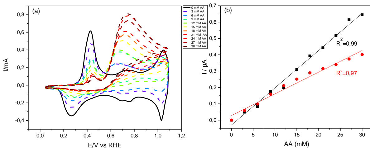
Figure 3.15 (a) cyclic voltammograms recorded during AA oxidation using a Pt electrode covered with Pani prepared in 1 M of \text{HClO}_4 at 1.2V. AA concentration range from 3 to 30 mM. (b) Calibration curves obtained with a Pt electrode covered with Pani obtained at 1.2V (black) and at 1.4V (red). v = 50 \text{ mV s}^{-1} in all cases.
