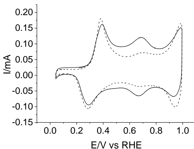
Figure 3.6. Electrochemical response in 1 M of HClO 4 medium of a Pt electrode covered with either polyaniline (dashed line) or an aniline–piperazine copolymer (ANI/PIP=0.2)
