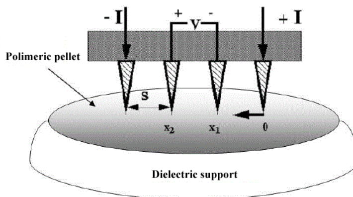
Figure 2.5: Conductivity measurement with the methods of four-points in line.
